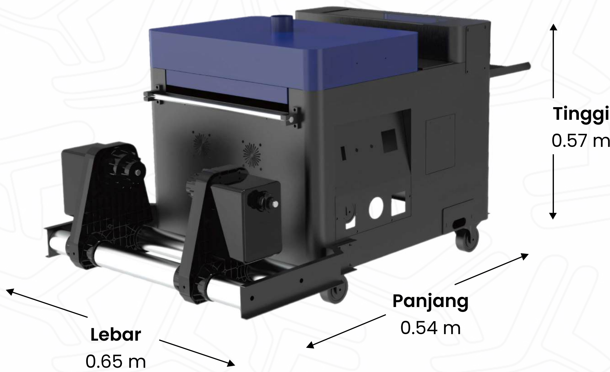
Ukuran Mesin Powder Shaker & Dryer (Curing)
